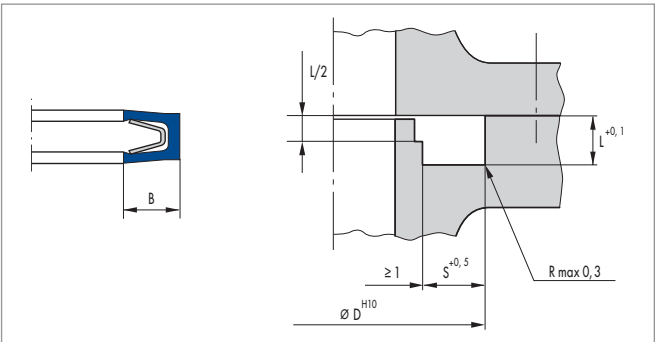
Installation example
