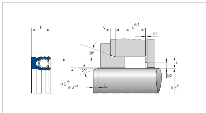
Installation example
