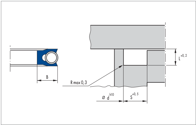
Installation example
